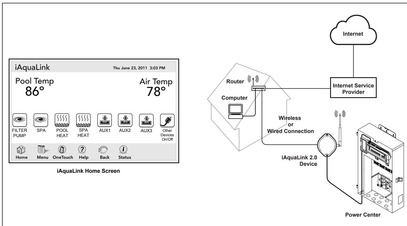
Figure 1. iAquaLink 2.0 Web Connect Device
